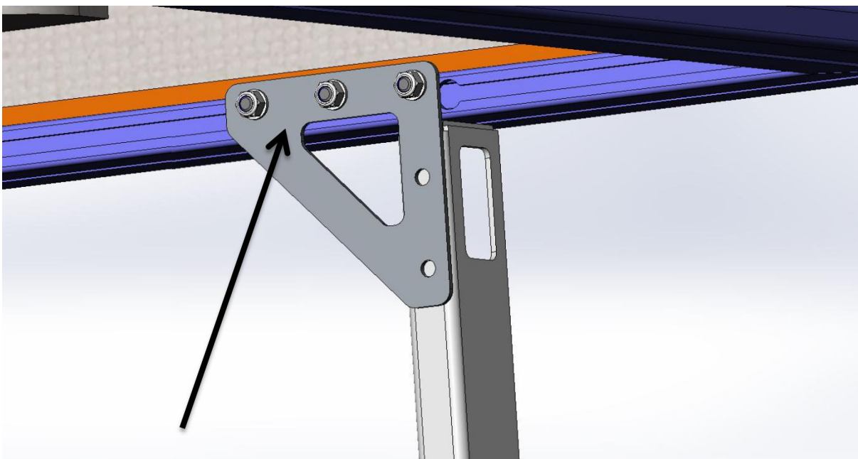
Figure 9: Hex Nuts inserted into the Canopy Camper Nut Slot, you can now place the the Bracket over these exposed Hex Nuts
