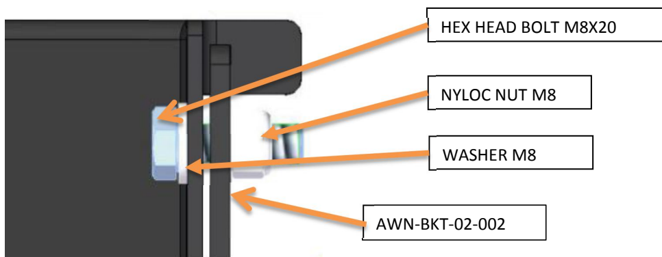
Figure 11: Front Mount Bolt Assembly
