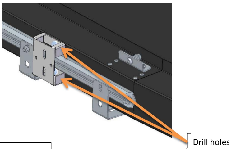
Figure 15:Rear Mount Position
